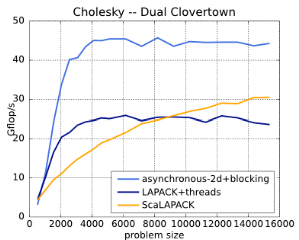
Figure 2. Comparison of parallelization techniques for Cholesky (Dual 4 core Intel Clovertown)
