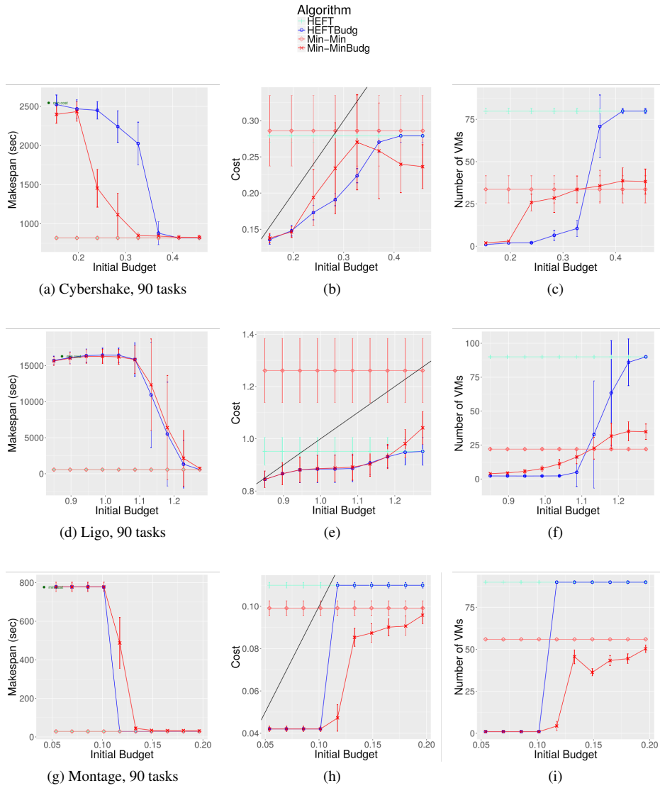
Figure 1: MIN-MIN, HEFT, budget-aware extensions MIN-MINBUDG and HEFTBUDG for the three workflow types with 90 tasks.
