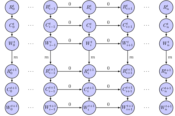
Figure 8: Task graph for 1D Gauss-Seidel. Here t is the iteration index, i the tile index and m the tile size.
