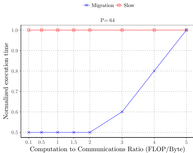
Figure 10: Performance of a 1D stencil according to the model with 64 threads.
