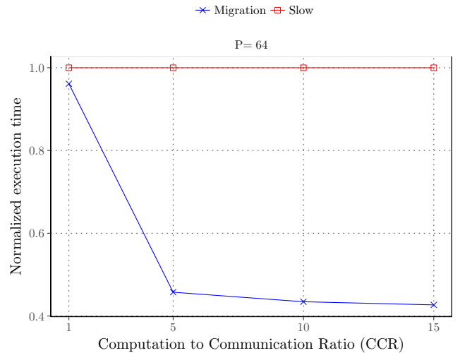
Figure 9: Performance of a 1D stencil running on a KNL with 64 threads.
