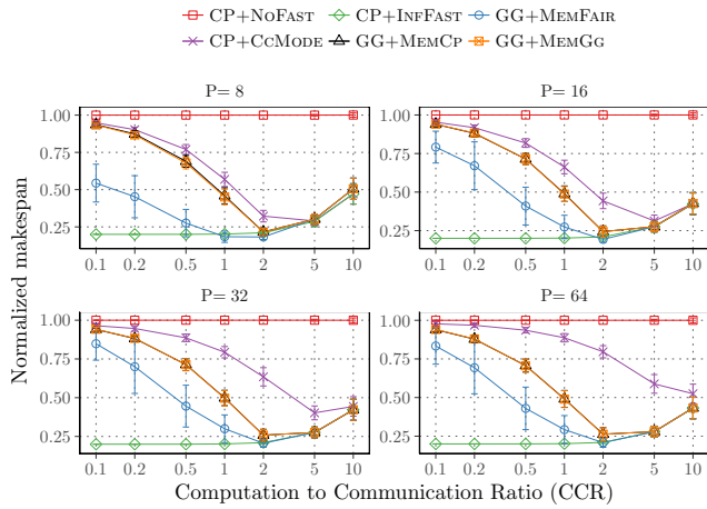
Figure 5: Impact of the number of processors with 50 node graphs and S_f = 1\text{GB} fast memory for GG processor scheduling heuristic.
