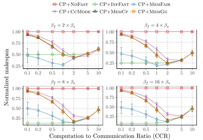
Figure 7: Impact of fast memory bandwidth with 50 nodes graph, 8 processors and S_f = 1\text{GB} .
