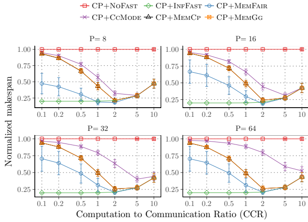
Figure 4: Impact of the number of processors with 50 nodes and S_f = 1\text{GB} fast memory with CP processor scheduling heuristic.
