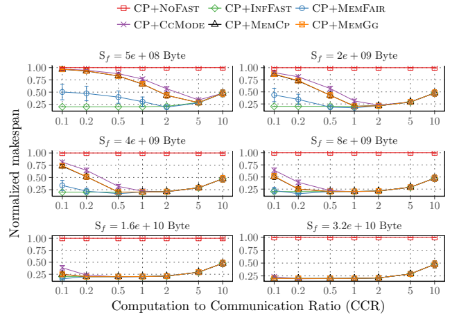
Figure 6: Impact of fast memory size with 50 node graphs and 8 processors.
