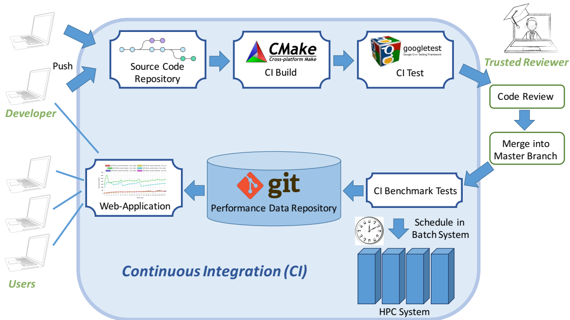
Figure 1: The software development ecosystem of the GINKGO library.
